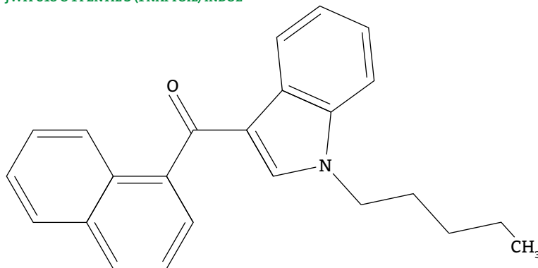
JWH 018 O 1 PENTIL 3 (1 NAFTOIL) INDOL
